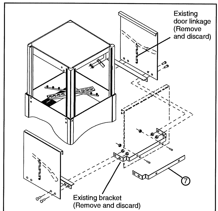
Figure 3 - Change the Door Lift Bracket
