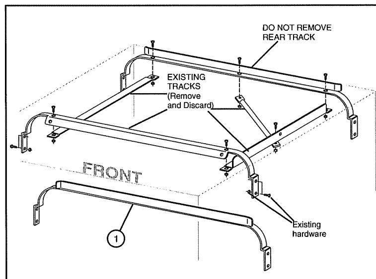
Figure 1- Change the Tracks
