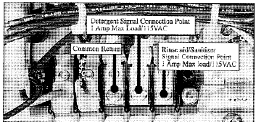
Figure 9 Chemical Signal Connection Points
