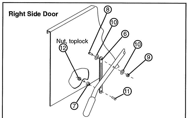
Figure 4 - Install the Door Lift Bar Assembly
