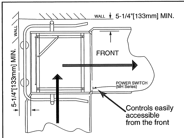
Figure 1- Machine Orientation for Corner Operation
