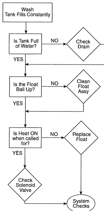
Figure 16 Float Switch Troubleshooting Chart
