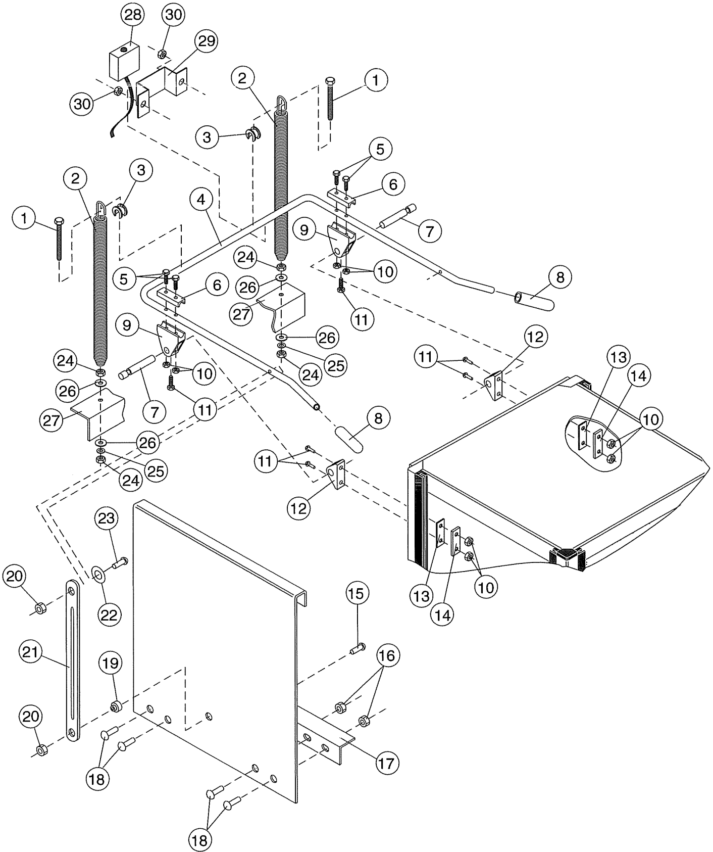
Figure 22 - MH-60/6N/6L Door Handle, Spring Assembly, and Safety Switch
