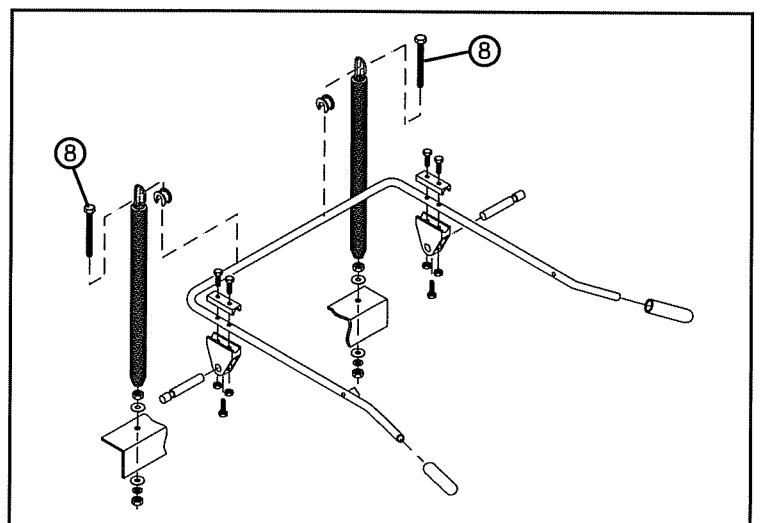
Figure 4 - Change the Extension Bolts
