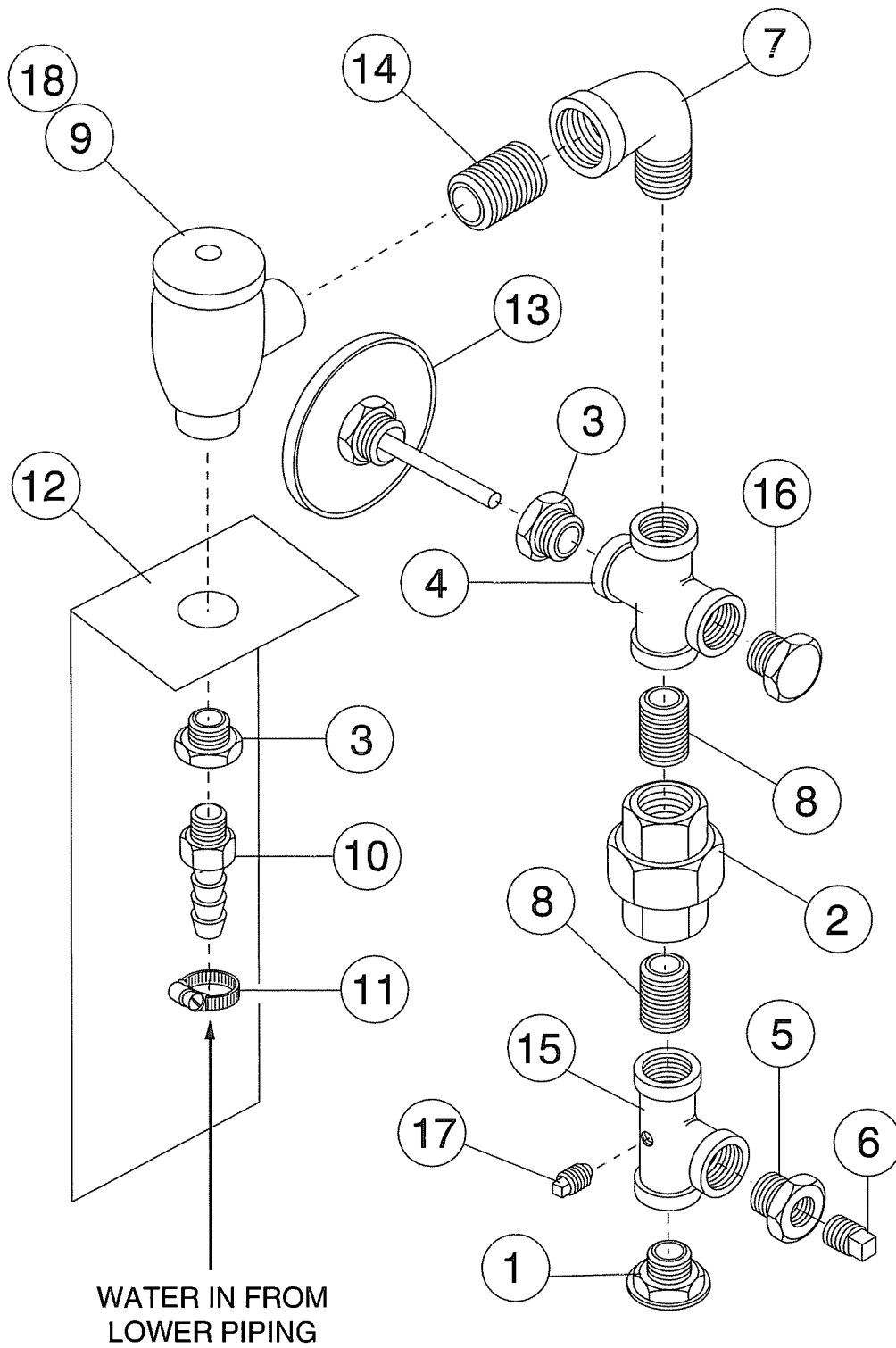
Figure 32 - MH-6L Only Upper Fill Piping Assembly
