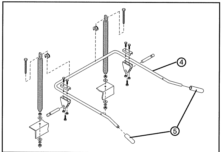
Figure 3 - Change the Door Handle
