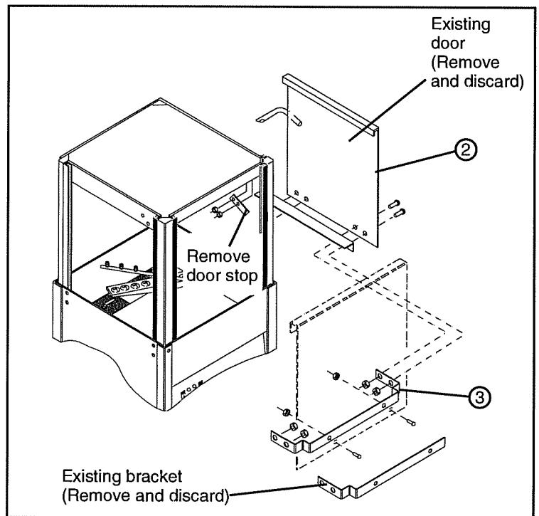
Figure 2 - Change Door and Door Lift Bracket
