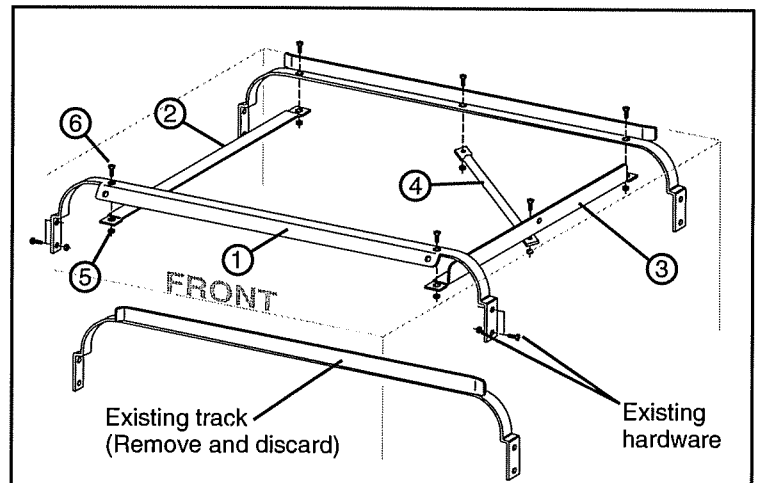
Figure 2 - Change the Tracks
