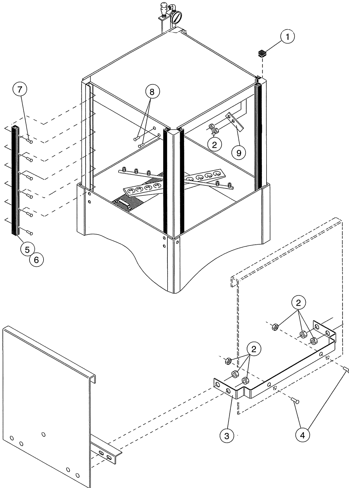
Figure 21 - MH-60/6N/6L Door Guides, Stops, and Lift Bracket
