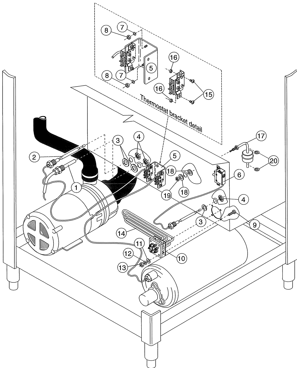
Figure 27 - MH-60/6N/6L Wash Tank Heat and Thermostats
