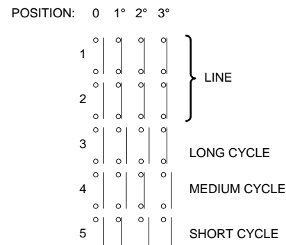
Q1 MAIN ROTARY SWITCH
